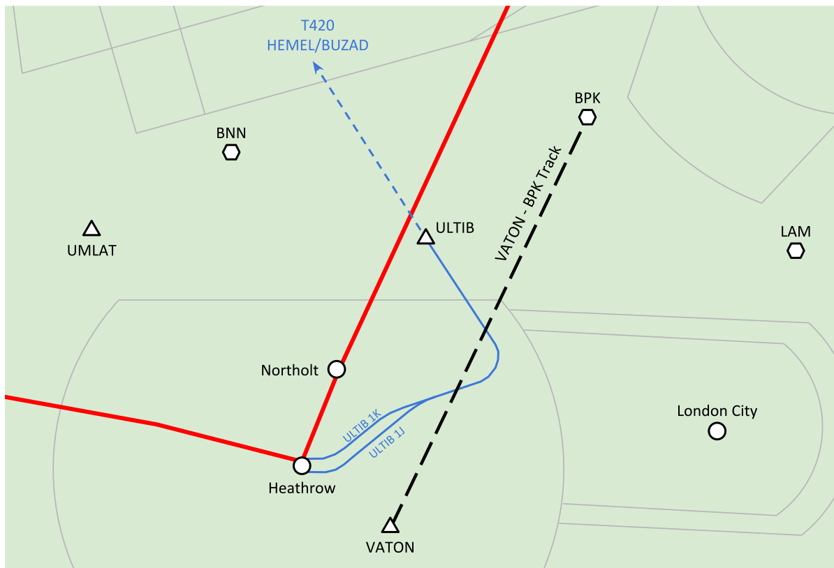
Figure LTC-3 – TC NW climb restrictions on ULTIB SIDs
