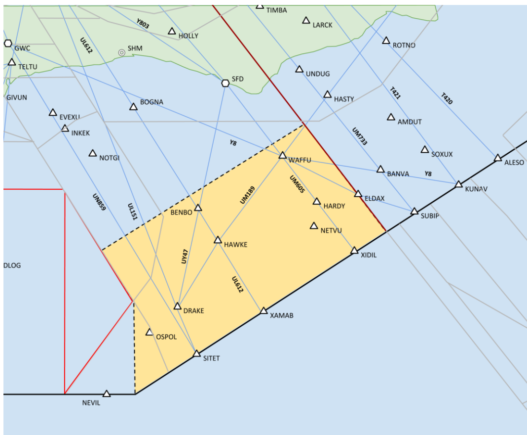
Figure LAC-4 – DIKRO Box
